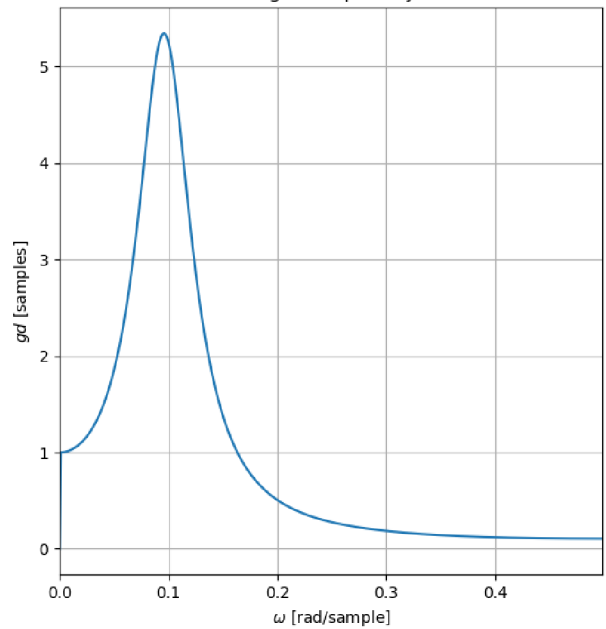
Lag / Group Delay
