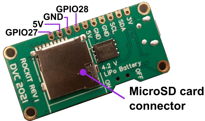
Fig.2. Bottom Rokit layout the general-purpose input/output pins (GPIO) 28 and 27 are used in the firmware to control servo motors 1 and 2 respectively. The I2C pins SDA and SCL corresponds to GPIO pins 10 and 11.
