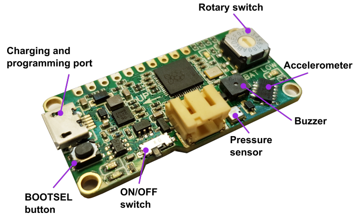
Fig.1. Top Rokit layout, the I2C pins as well as the servo signal pins operate at 3.3 V. Connecting these pins to a 5V signal source will destroy the microcontroller. For best data logging speed, use a class-10 microSD card.
