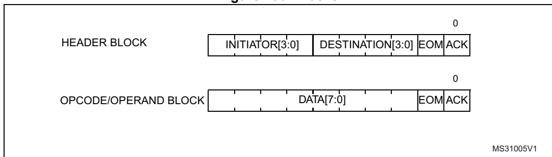
Figure 286. Blocks
