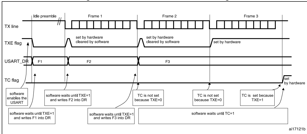
Figure 201. TC/TXE behavior when transmitting
