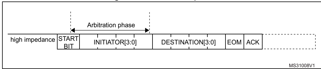
Figure 289. Arbitration phase
