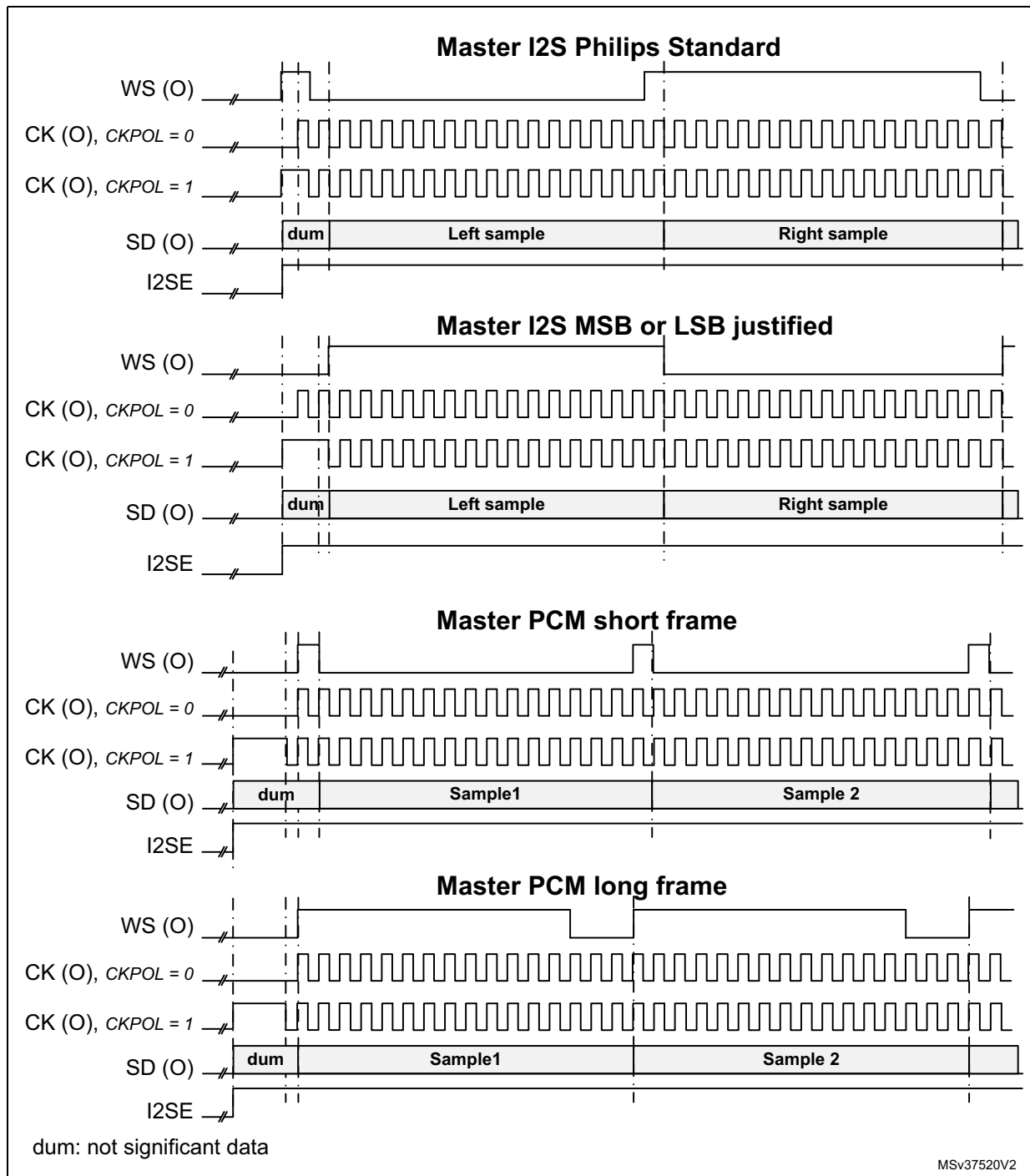
Figure 258. Start sequence in master mode
