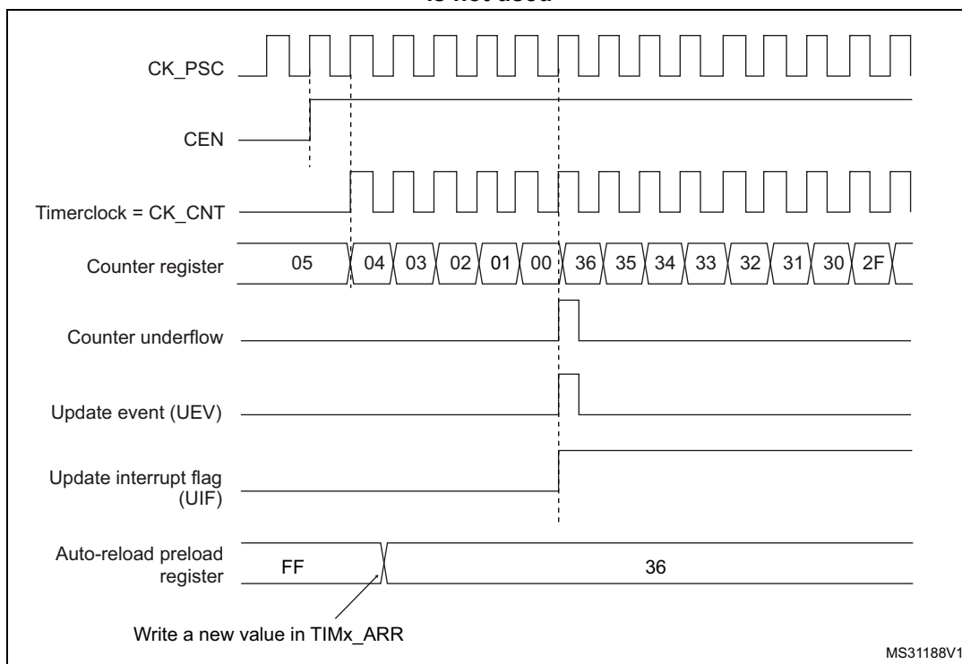
Figure 67. Counter timing diagram, Update event when repetition counter is not used
