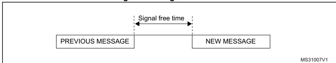
Figure 288. Signal free time
