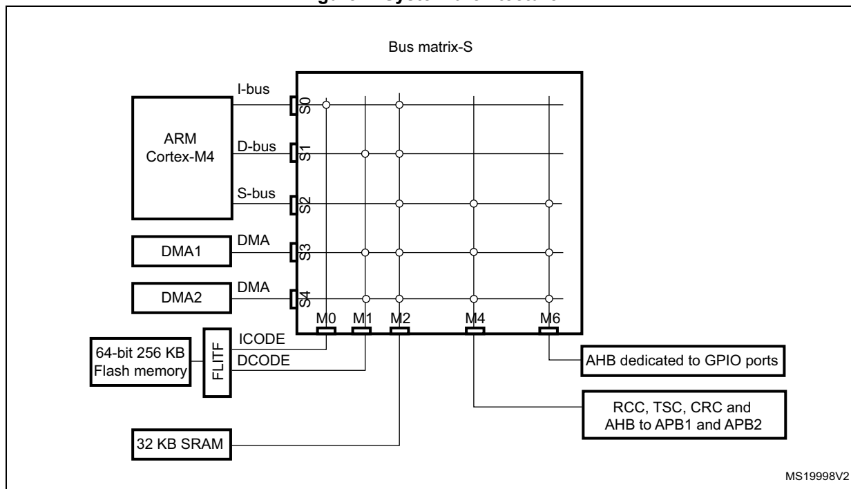
Figure 1. System architecture
