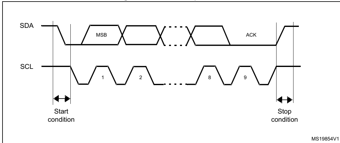
Figure 168. I 2 C bus protocol
