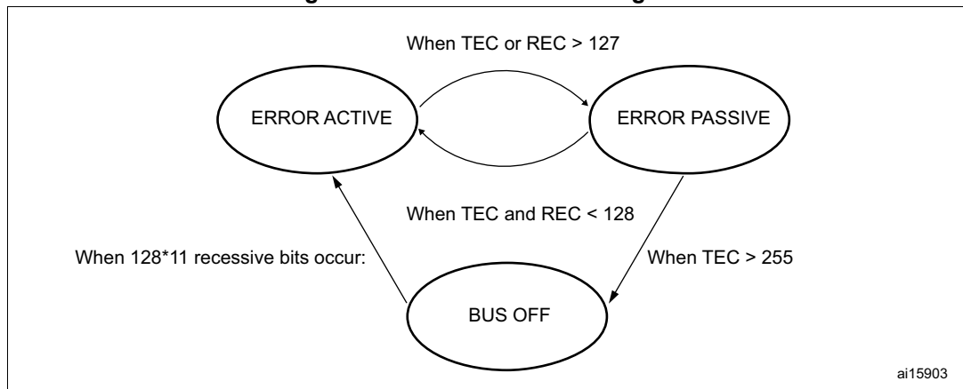
Figure 277. CAN error state diagram
