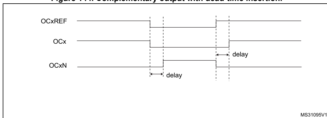
Figure 144. Complementary output with dead-time insertion.
