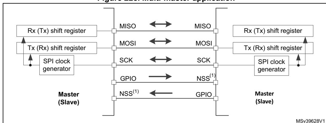
Figure 228. Multi-master application
