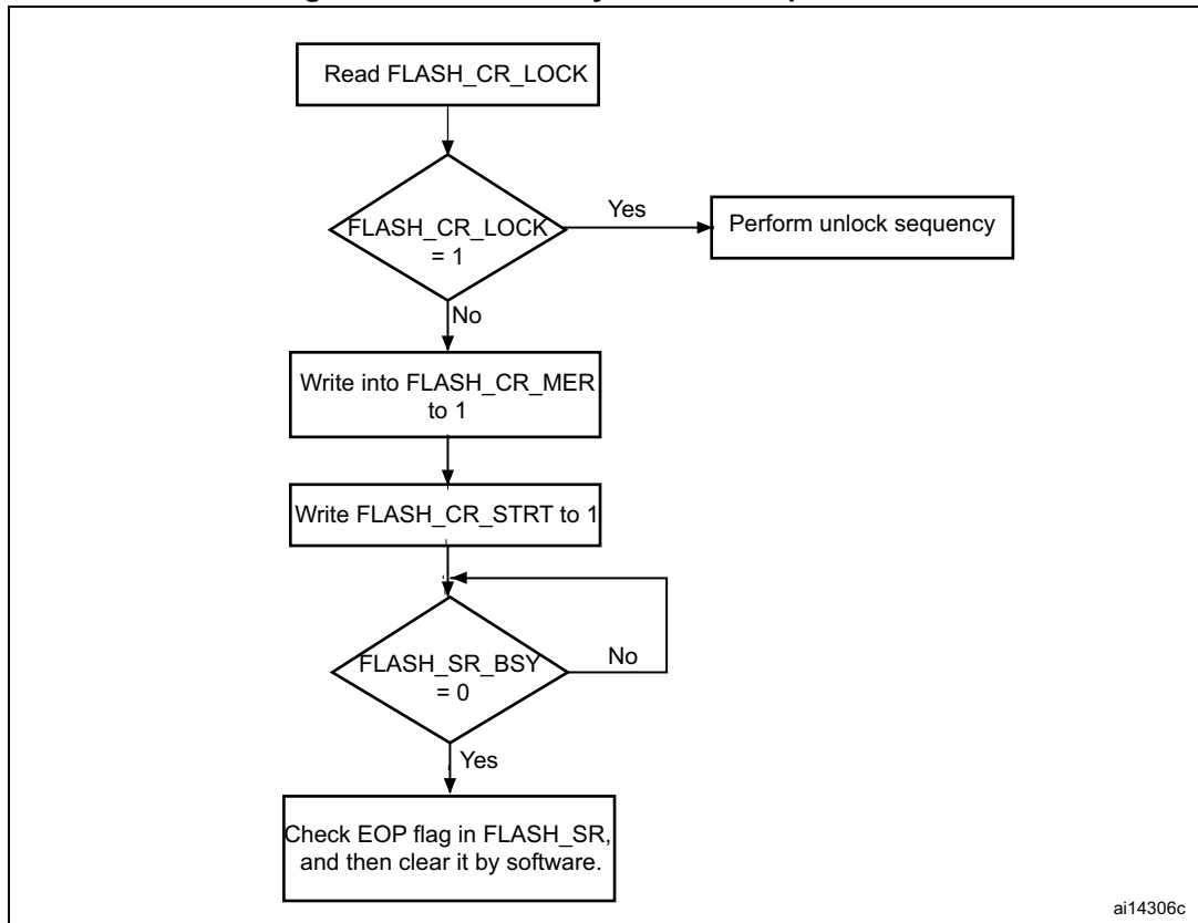
Figure 5. Flash memory Mass Erase procedure
