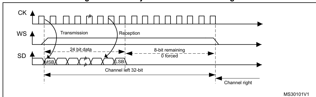
Figure 248. MSB justified 24-bit frame length
