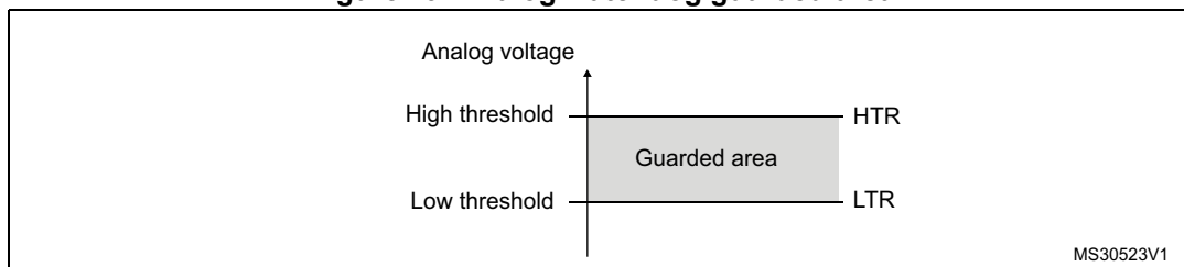
Figure 29. Analog watchdog guarded area
