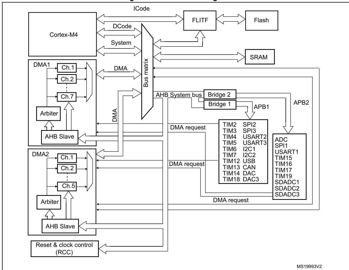
Figure 24. DMA block diagram
