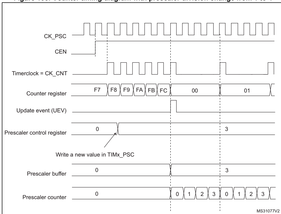
Figure 103. Counter timing diagram with prescaler division change from 1 to 4
