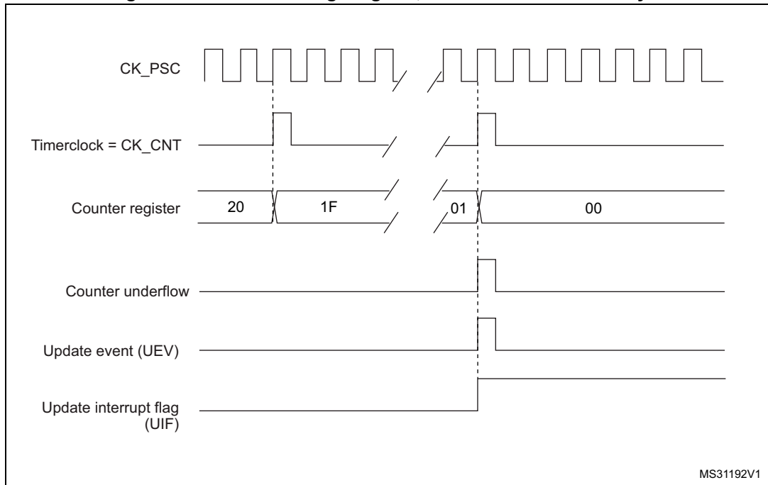
Figure 72. Counter timing diagram, Update event with ARPE=1 (counter underflow)
