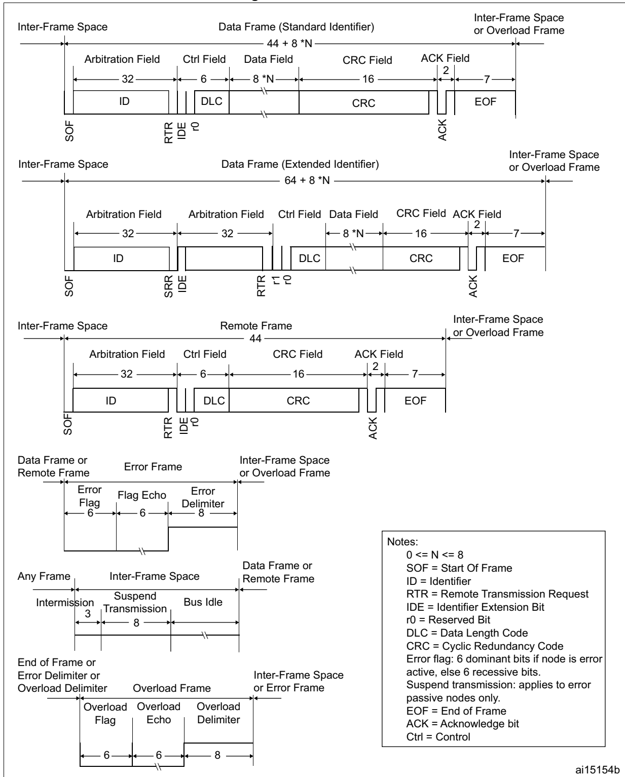
Figure 279. CAN frames
