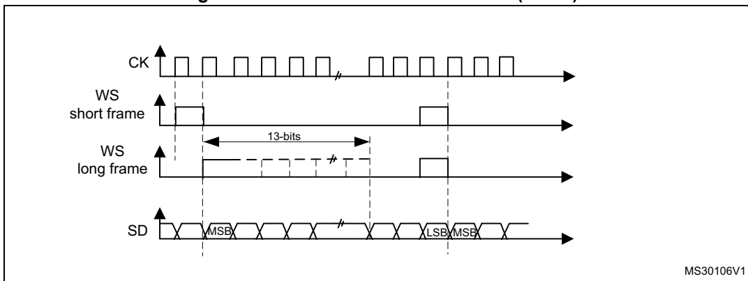
Figure 256. PCM standard waveforms (16-bit)
