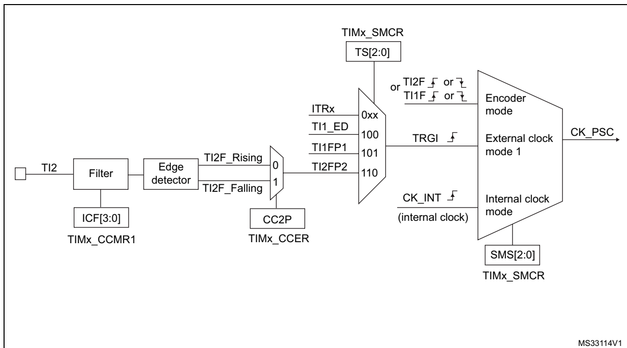
Figure 111. T12 external clock connection example
