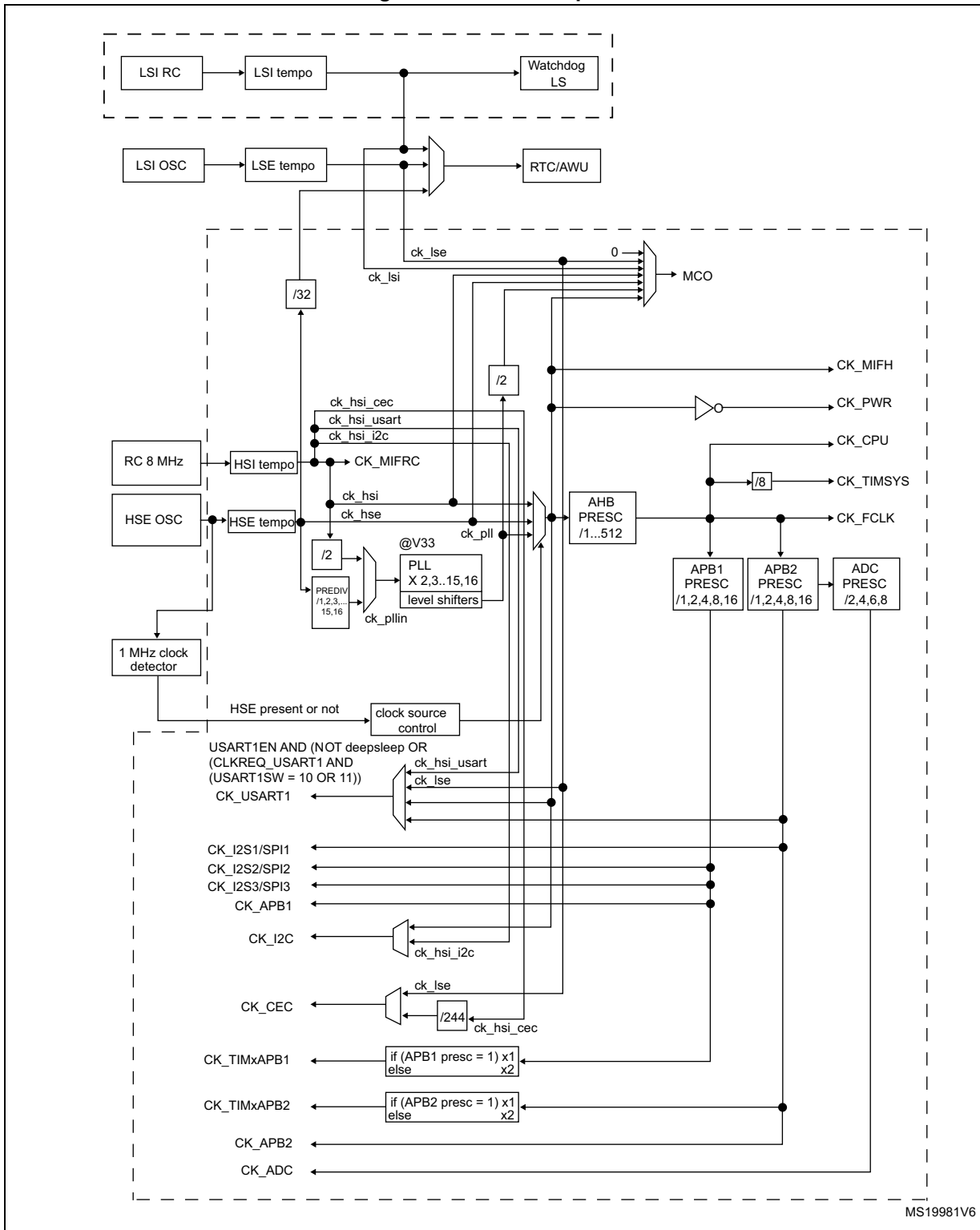
Figure 12. Clock tree part 1
