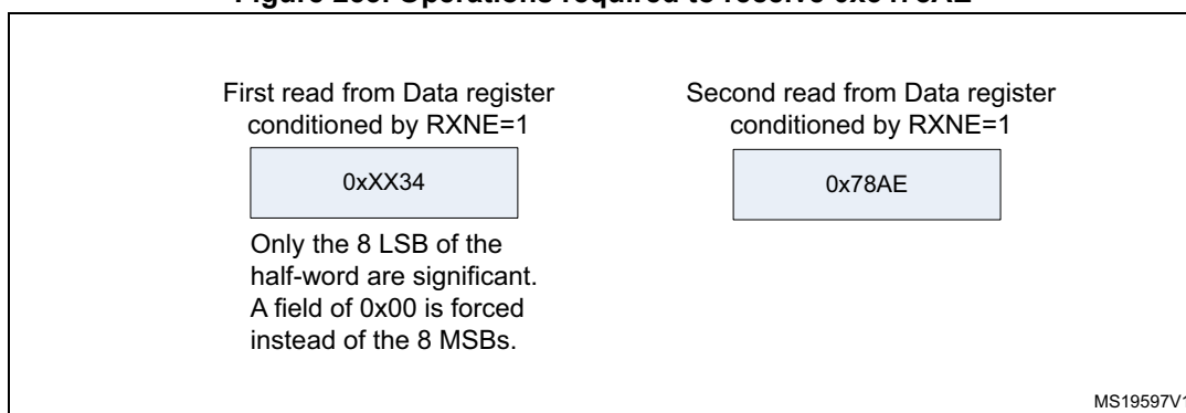
Figure 253. Operations required to receive 0x3478AE
