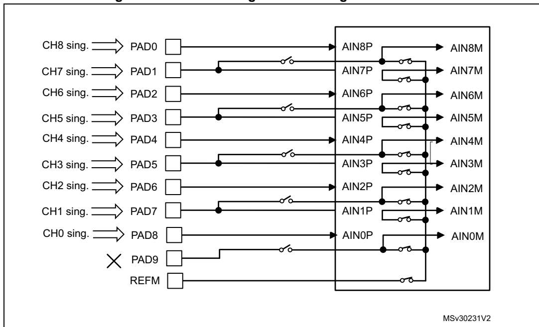
Figure 37. Switch configuration in single-ended mode
