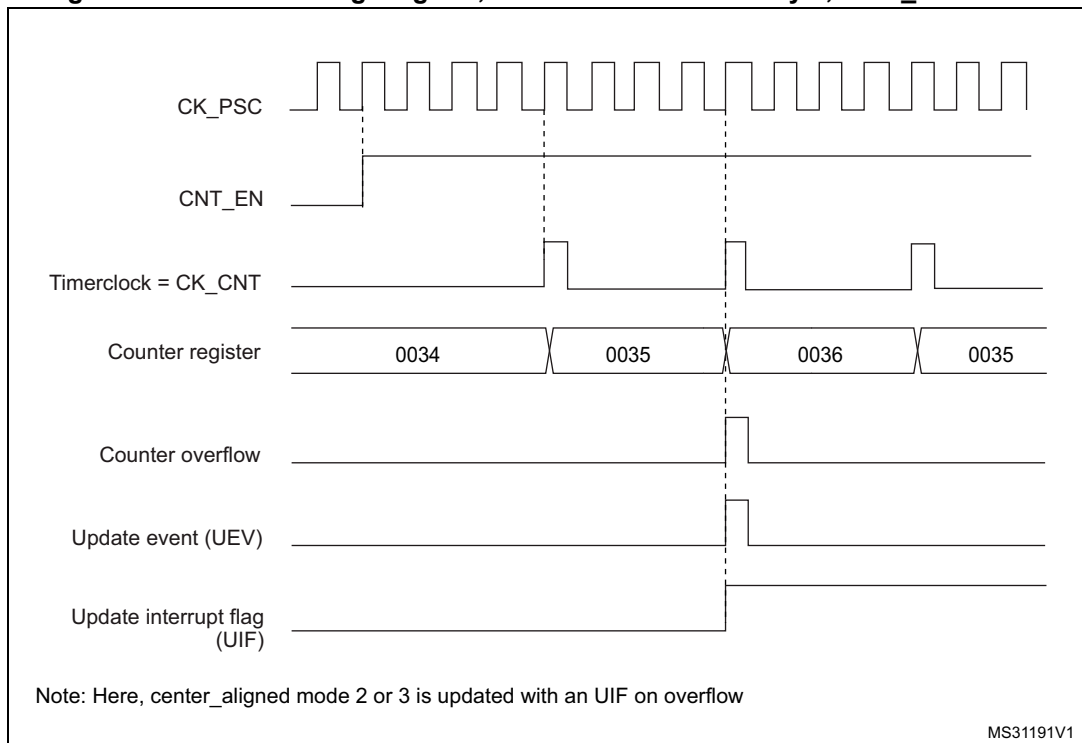
Figure 70. Counter timing diagram, internal clock divided by 4, TIMx_ARR=0x36
