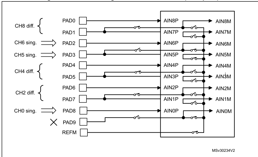
Figure 39. Switch configuration in mixed mode (example 1)
