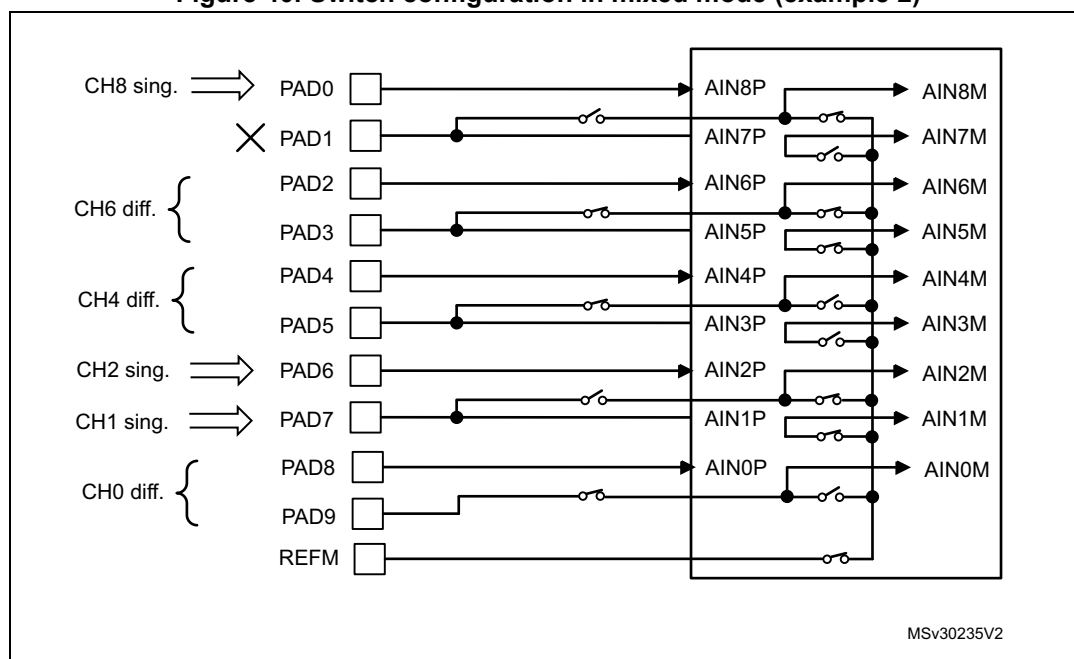
Figure 40. Switch configuration in mixed mode (example 2)
