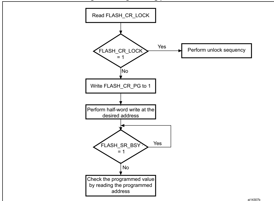
Figure 3. Programming procedure
