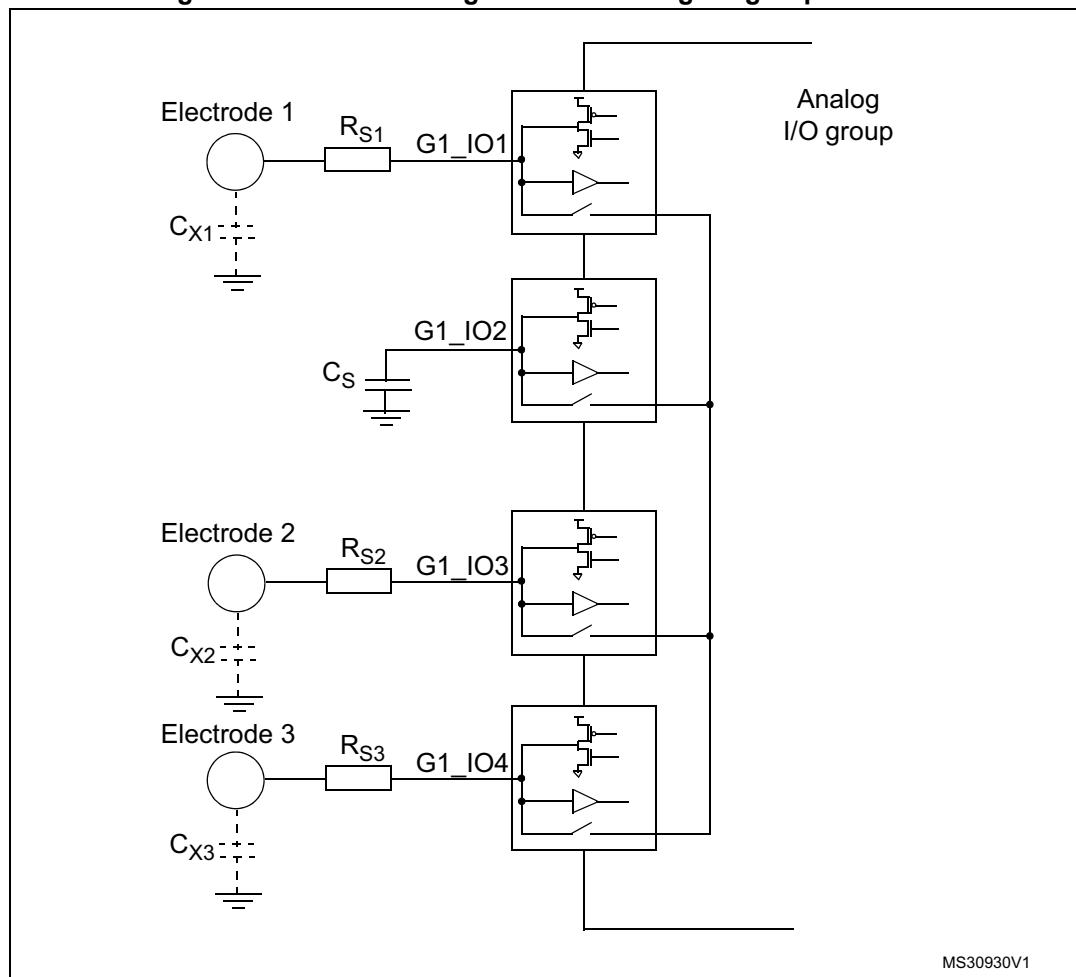
Figure 262. Surface charge transfer analog I/O group structure
