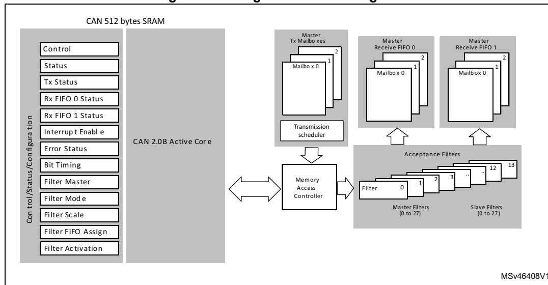
Figure 267. Single-CAN block diagram
