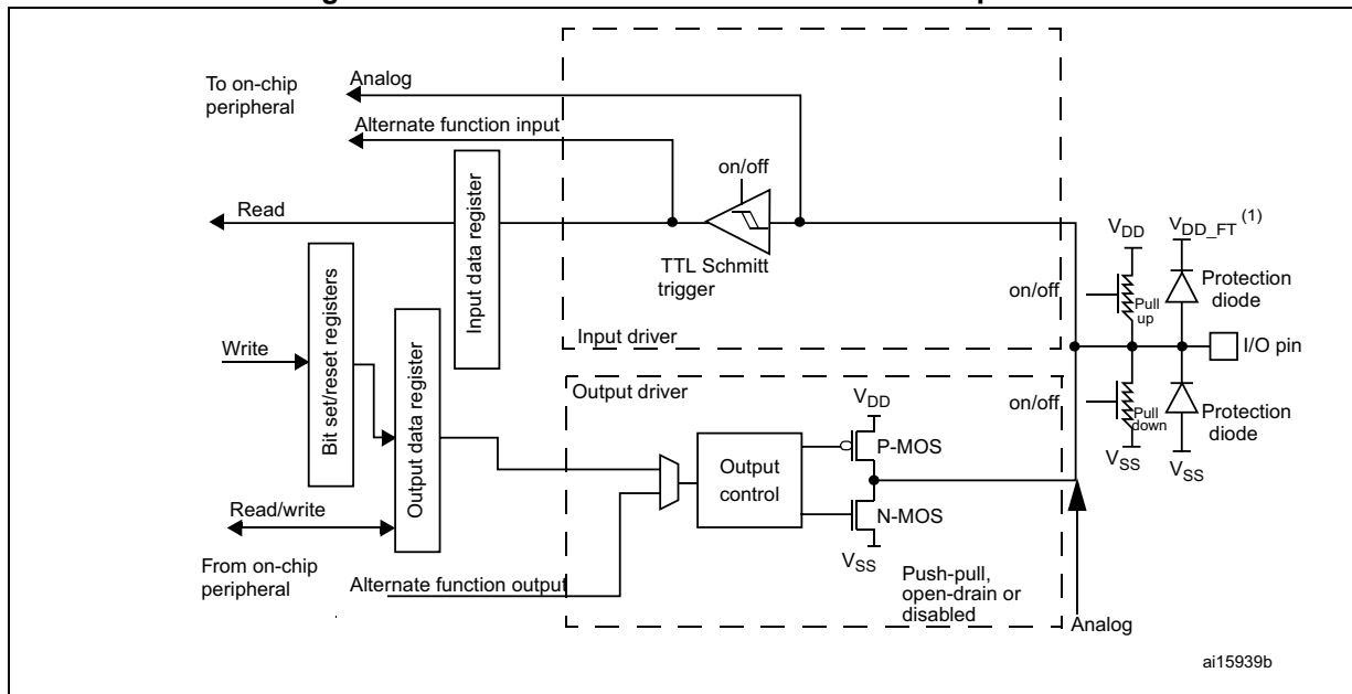
Figure 17. Basic structure of a 5-Volt tolerant I/O port bit
