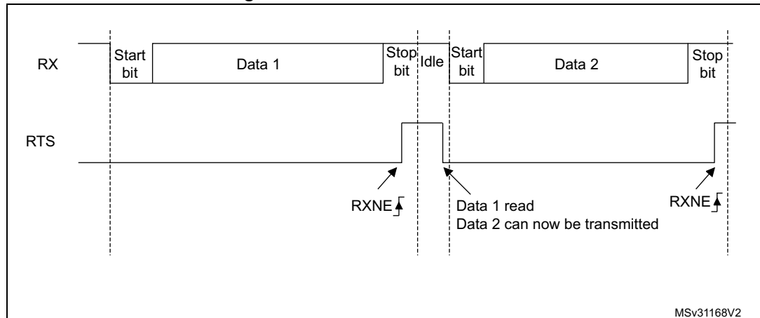
Figure 220. RS232 RTS flow control
