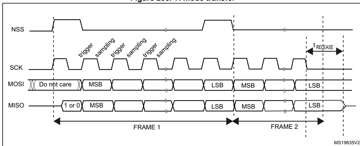
Figure 238. TI mode transfer
