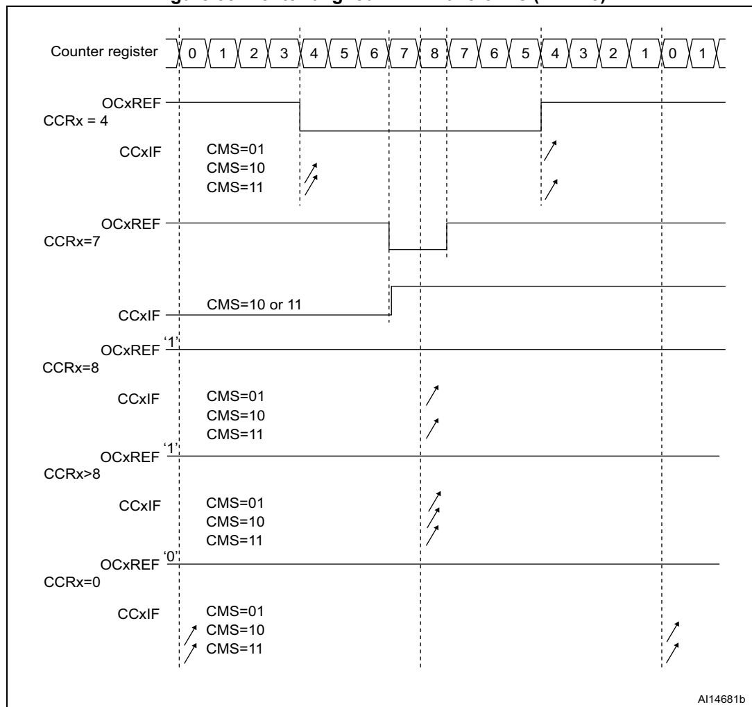
Figure 85. Center-aligned PWM waveforms (ARR=8)
