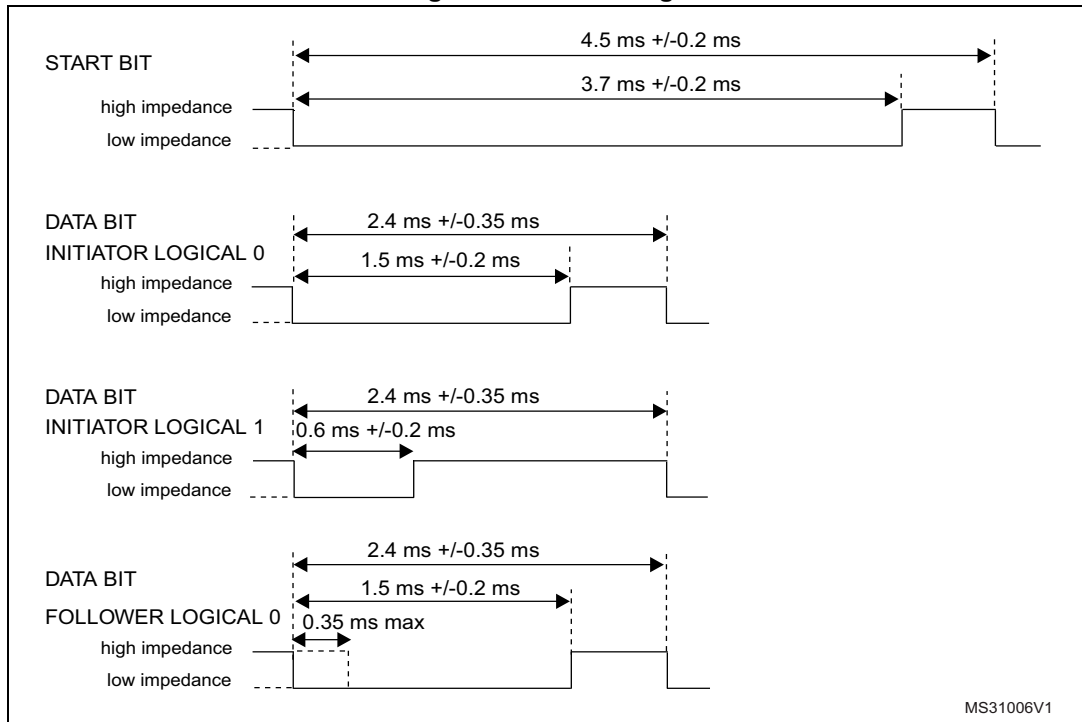
Figure 287. Bit timings
