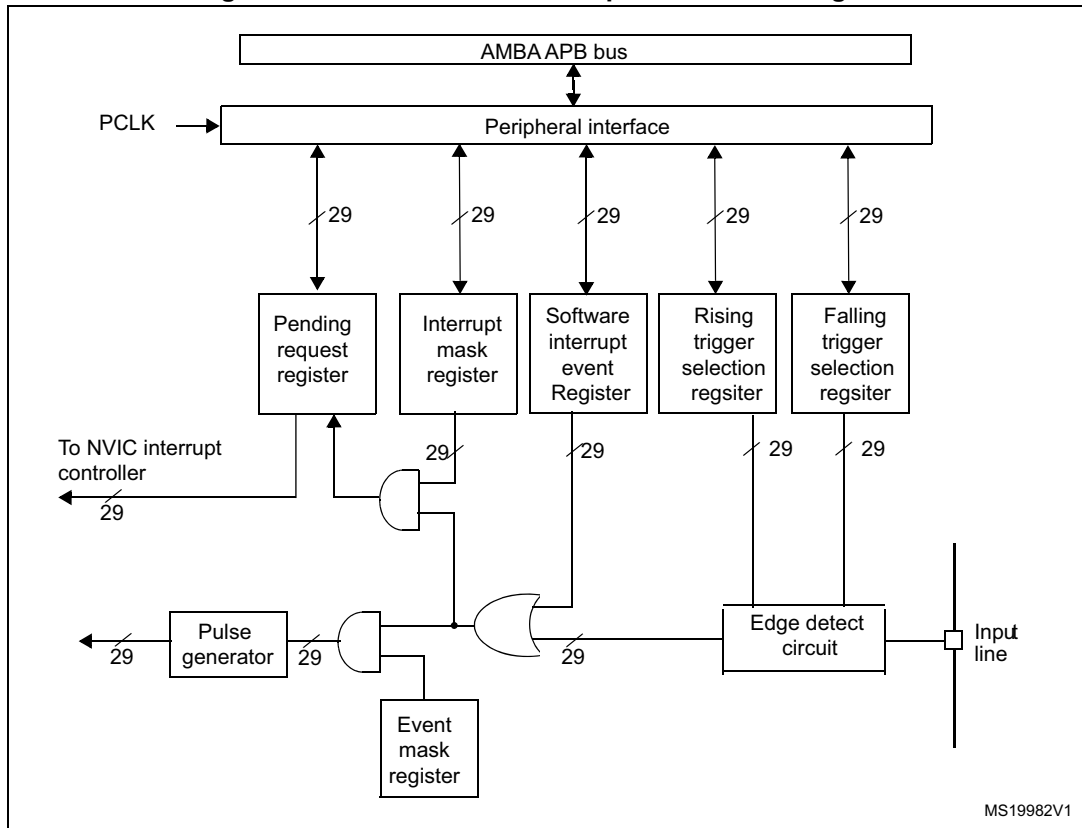
Figure 25. EXTI extended interrupt/event block diagram
