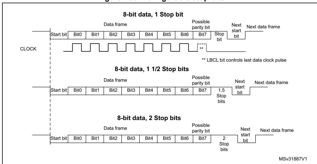
Figure 200. Configurable stop bits
