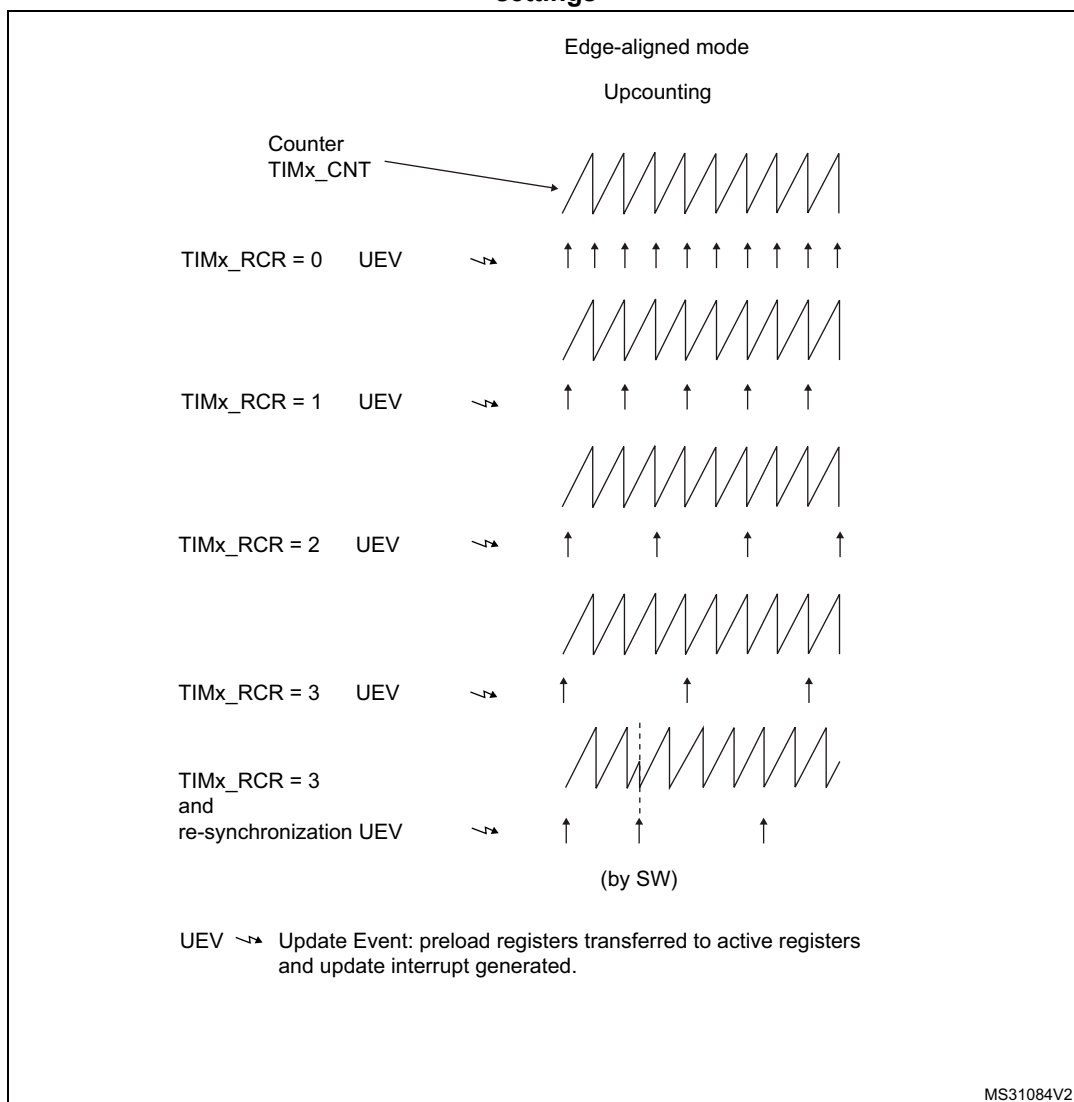
Figure 133. Update rate examples depending on mode and TIMx_RCR register settings
