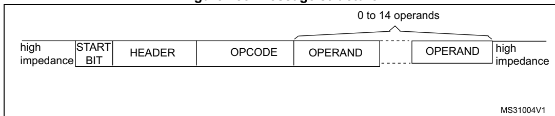
Figure 286. Blocks
