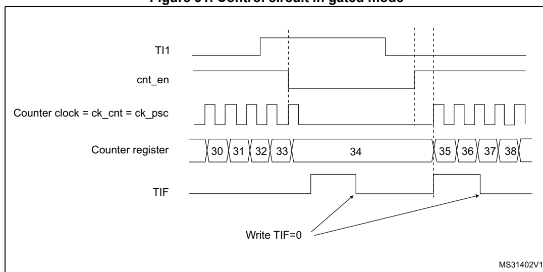
Figure 91. Control circuit in gated mode
