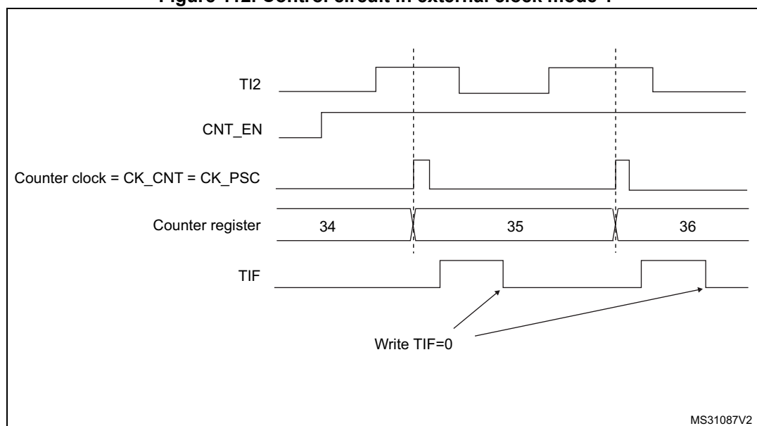
Figure 112. Control circuit in external clock mode 1
