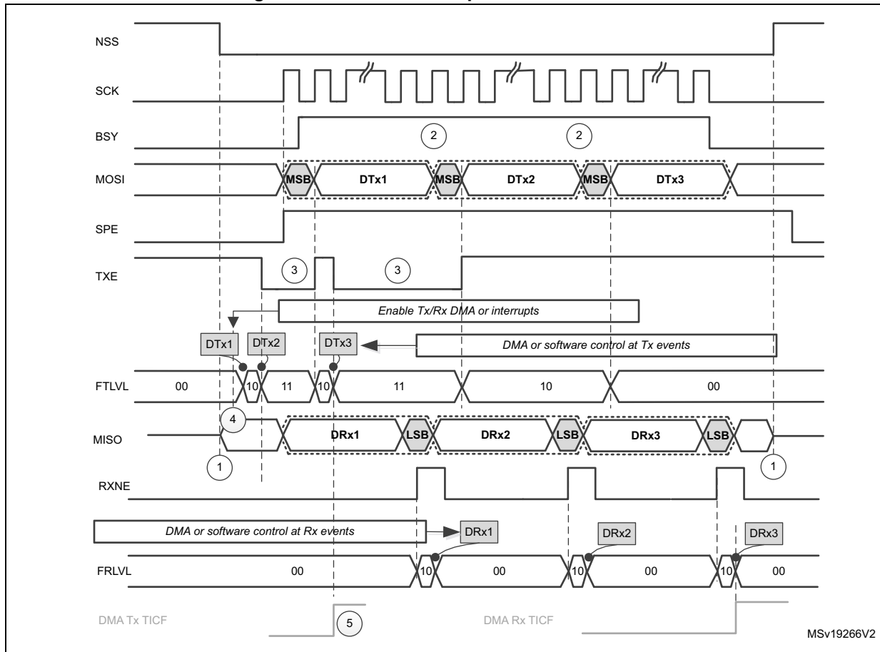
Figure 233. Master full-duplex communication
