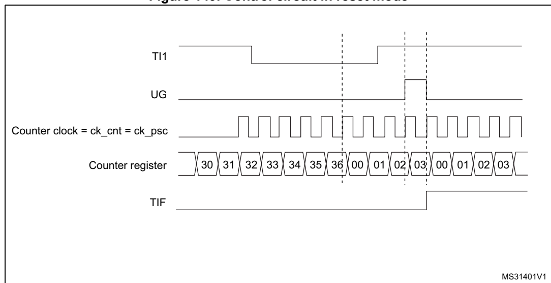
Figure 149. Control circuit in reset mode
