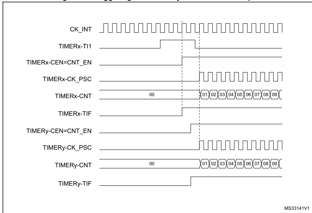
Figure 99. Triggering timer x and y with timer x T11 input
