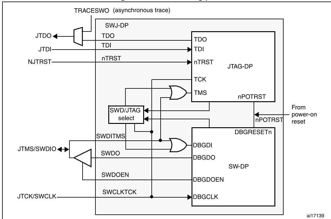
Figure 295 shows that the asynchronous TRACE output (TRACESWO) is multiplexed with TDO. This means that the asynchronous trace can only be used with SW-DP, not JTAG-DP.
