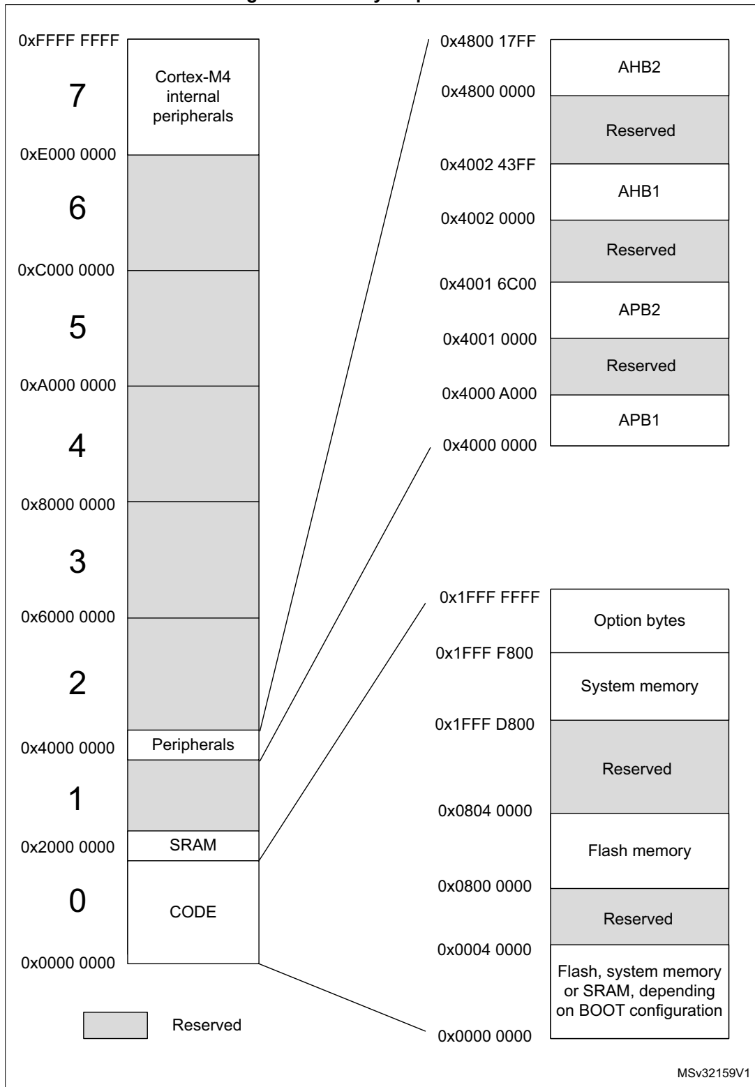
Figure 2. Memory map
