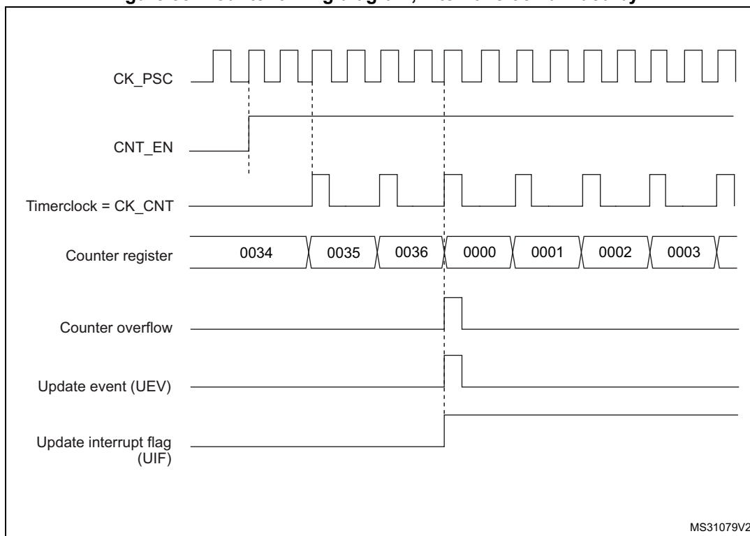
Figure 58. Counter timing diagram, internal clock divided by 2
